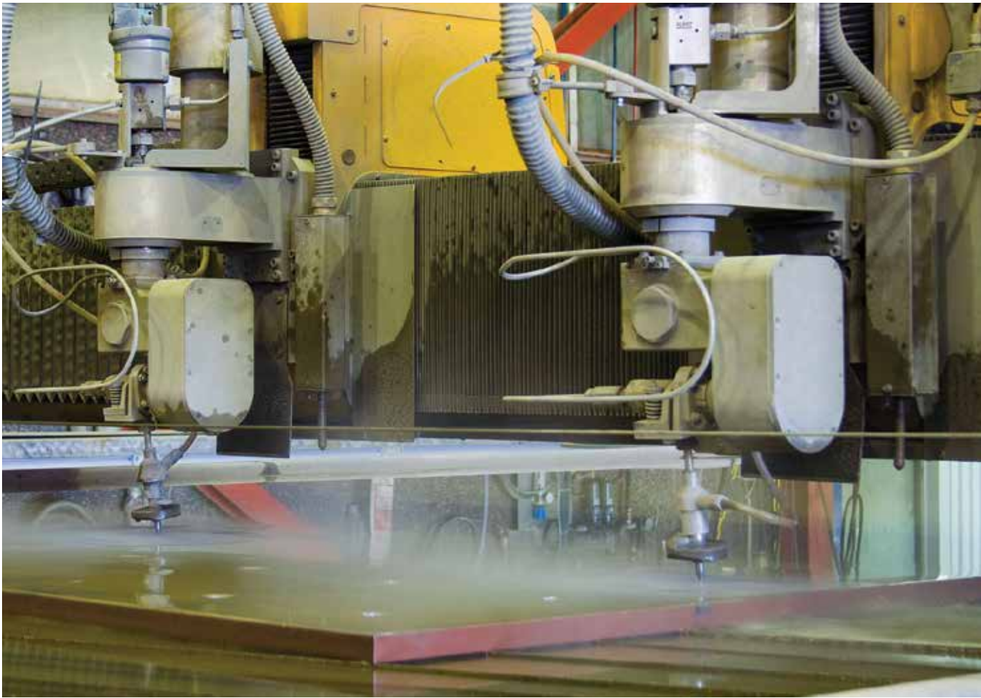
LKAB Mekaniska's 5-axis waterjet cutting machine.
